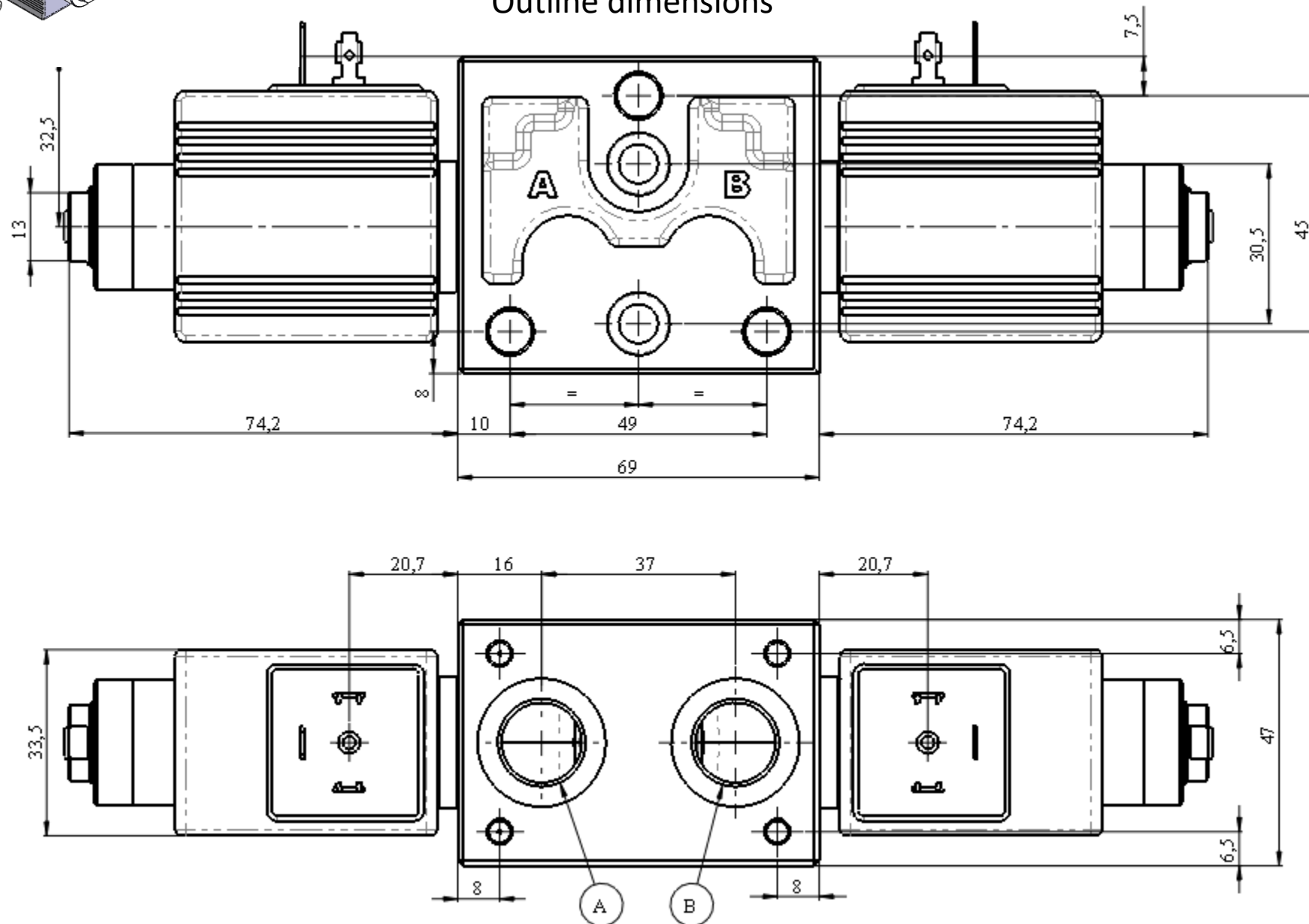
Outline dimensions
