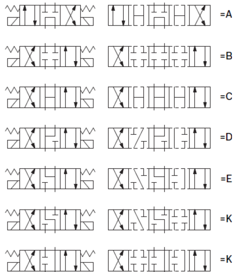
Spool schemes
